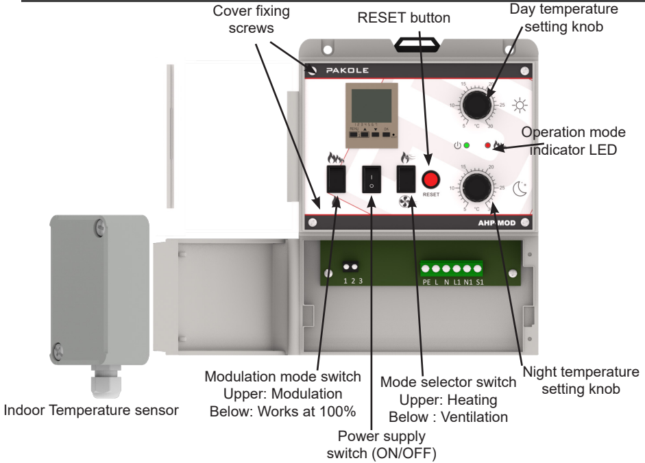
1/a. fig: Front view of the temperature regulator
