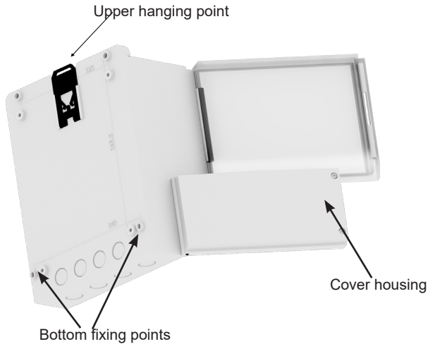
1/b. fig: Rear view of the temperature regulator
