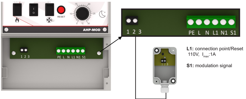
3. fig: Connection points of the temperature regulator (terminal strip)
